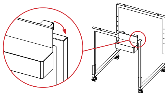
Mounting the SPEEDRAIL_30 at the frame of a STAGE table.
