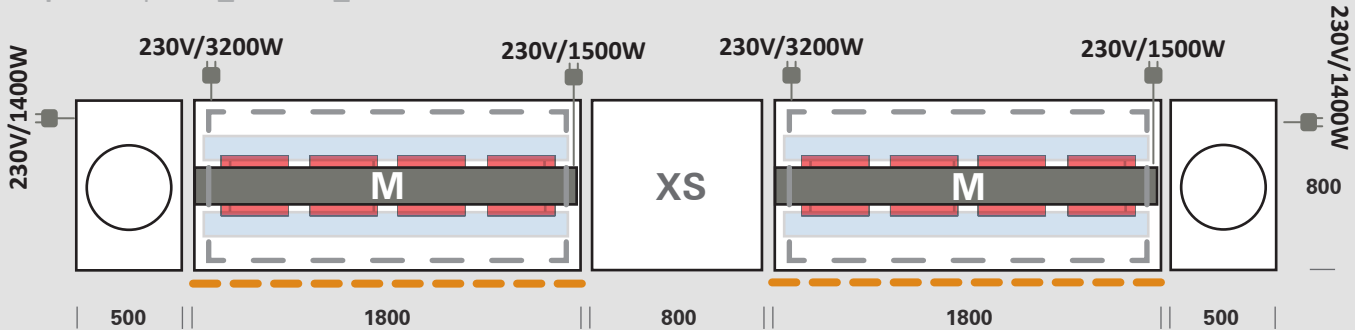
top view | HOT_BUFFERET_STATION
