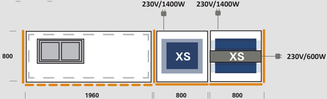
top view | SALAD_BREAD_STATION
