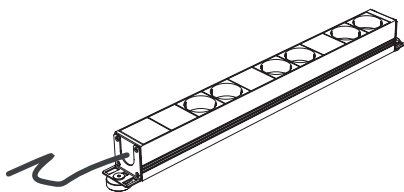
plugbar_CEE_400V_3x16A_3600W
